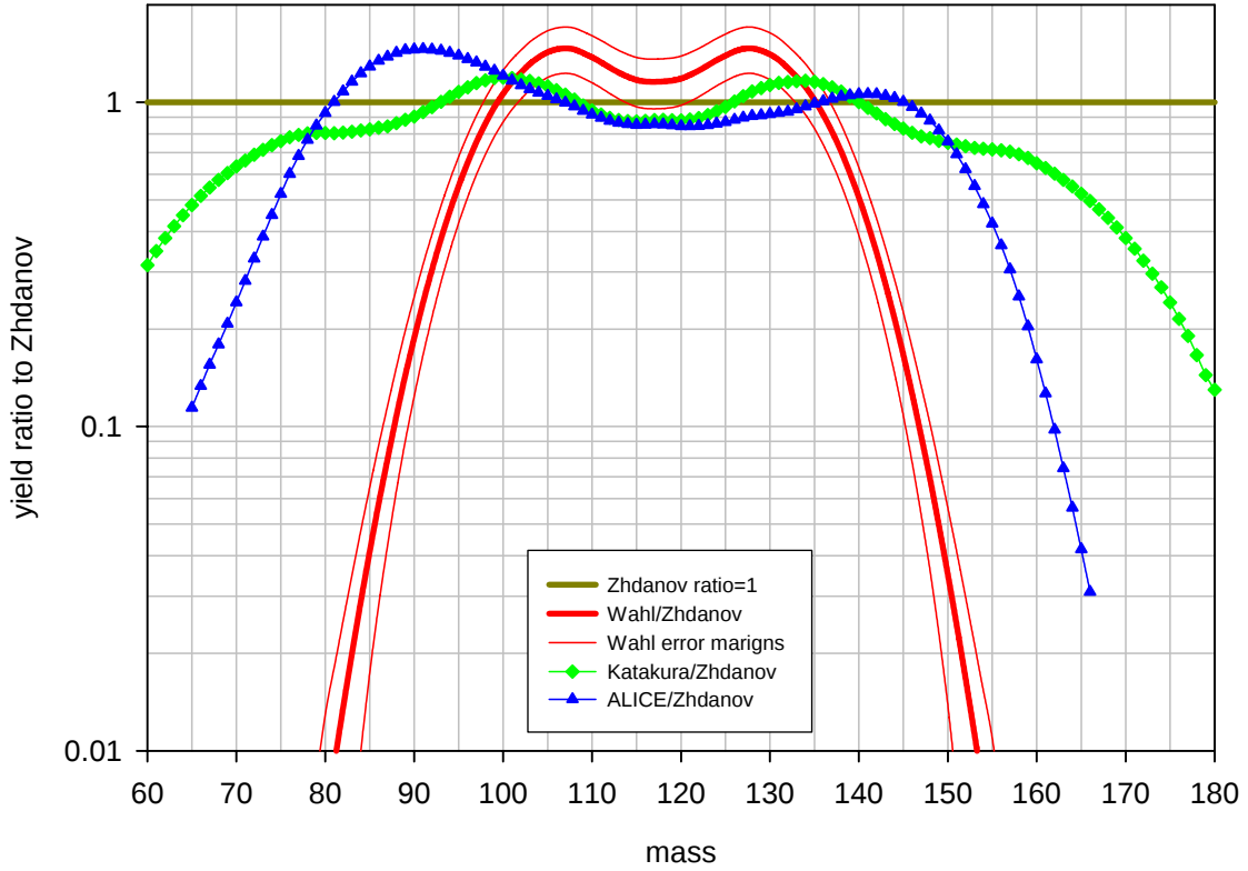
Benchmark B: ^{244}\text{Cm} at 100 MeV, post neutron emission yield ratios to Zhdanov's data
